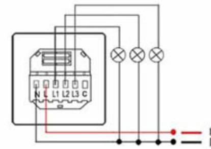
Light Switch
