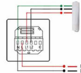
Curtain Switch
