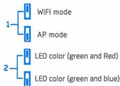
Encode structure
