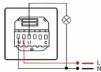
Dimmer Switch
