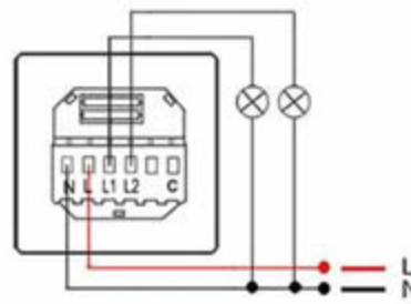
Light Switch
